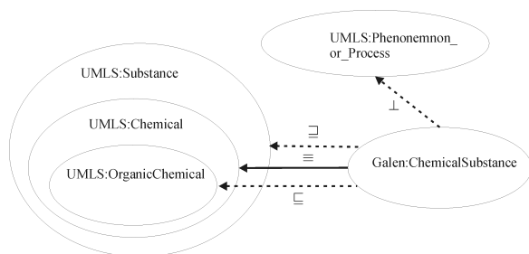
Figure 3: Derivation of additional Mappings
