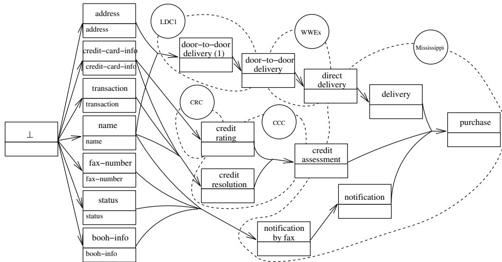
Figure 4: Minimum Decomposition Path
