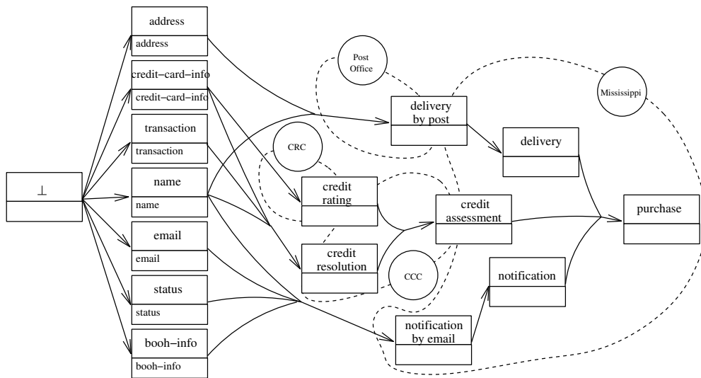
Figure 8: Minimum Decomposition Path
