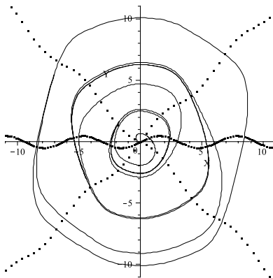
Figure 5: d(x) = \frac{\sin x}{2} .
